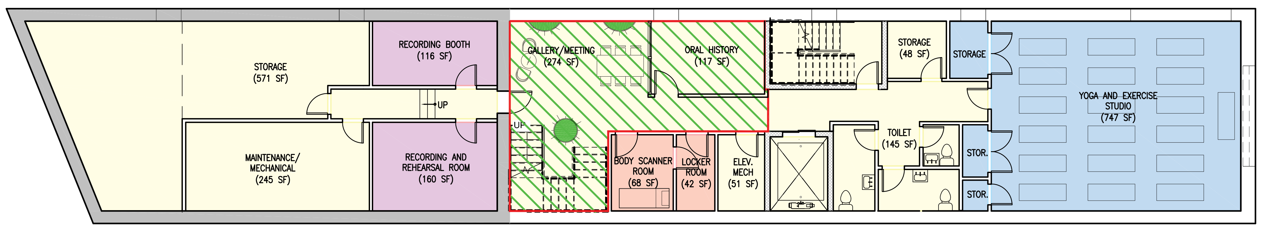
Basement Plan
